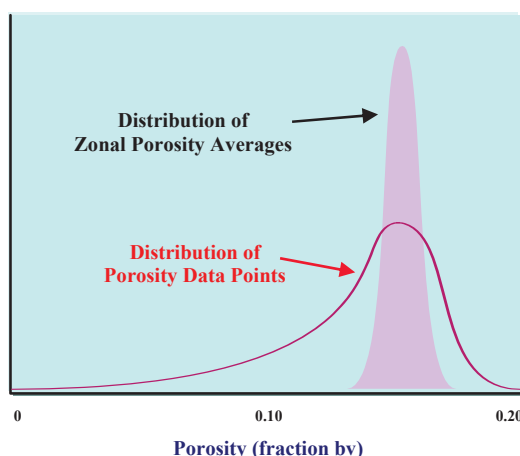
Fig. 5.5—Frequency distributions of porosity.
