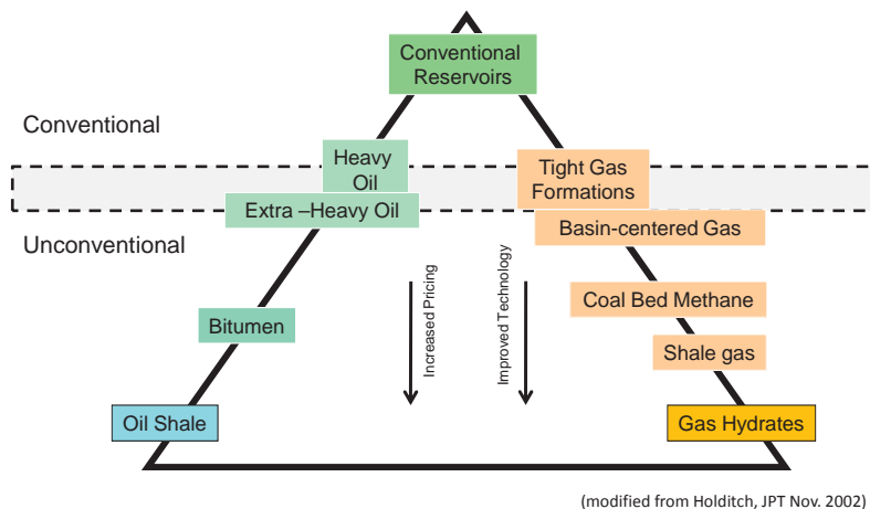
Fig. 8.1—Resource triangle.
