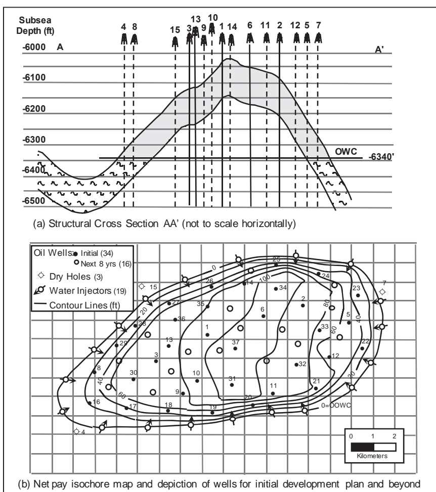
Fig. 4.5—Volumetric assessment of Reserves (initial development stage).
