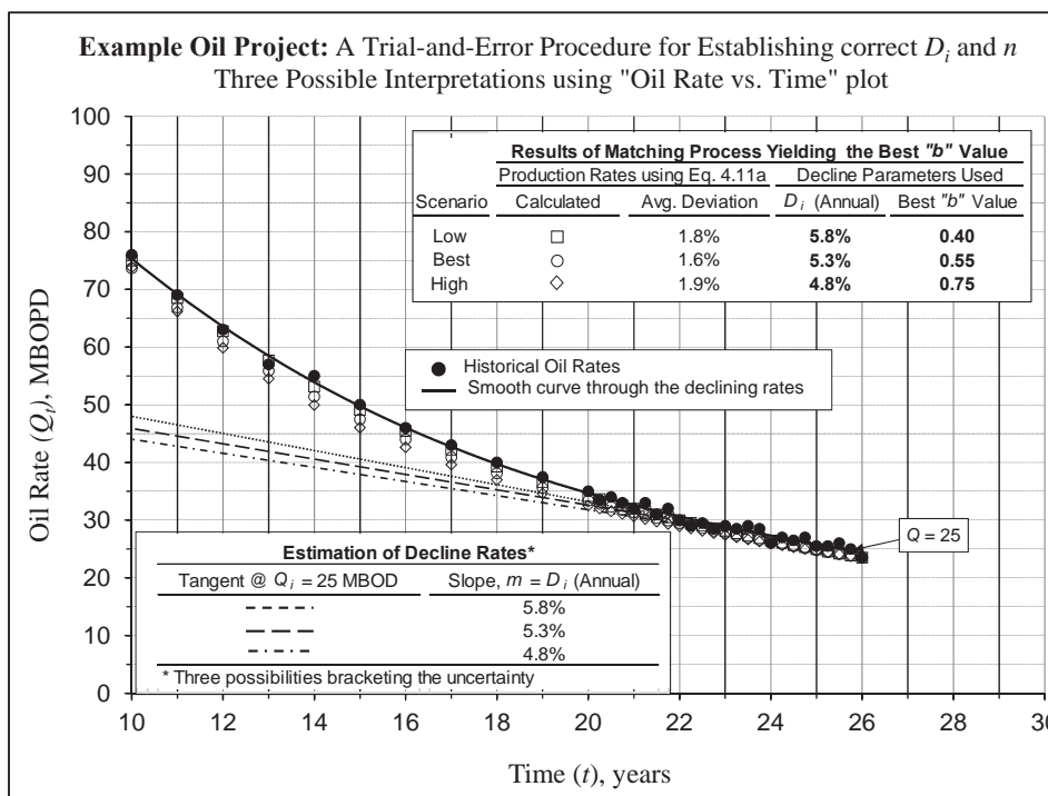
Fig. 4.10a—Estimation of hyperbolic decline parameters using rate vs. time plots.
