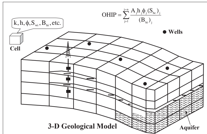
Fig. 4.6—3D multicell geological model [adapted from PS-CIM (2004)]
