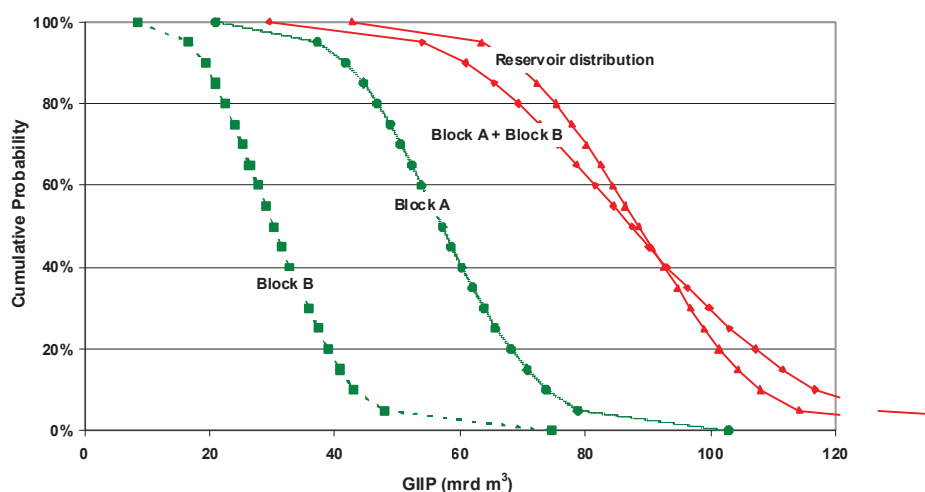
Figure 6.3—Probability Distribution—Reservoir Blocks A and B
