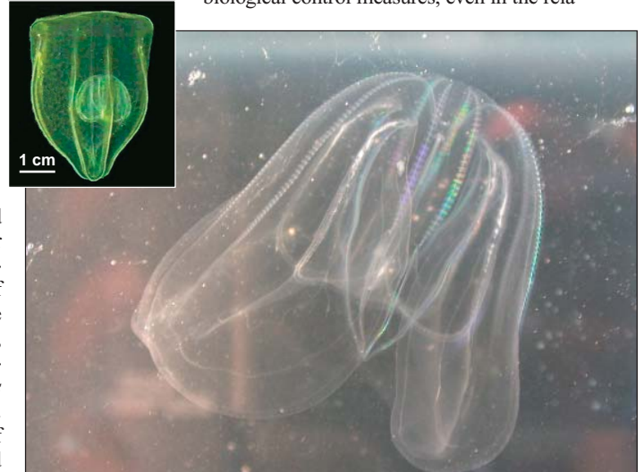
Invading the invader. (Bottom) The arrival of the Northwestern Atlantic ctenophore (comb jelly) Mnemiopsis in the Black Sea via the ballast waters of cargo ships in the early 1980s devastated the natural ecosystem of this marine environment. (Top) Beroe species of ctenophore are the natural predators of Mnemiopsis . The arrival of Beroe in the Black Sea in 1997 resulted in control of the Mnemiopsis population and contributed to recovery of the Black Sea ecosystem. In this photograph, a Beroe ctenophore has ingested the smaller Mnemiopsis , which is visible inside its gut cavity.
