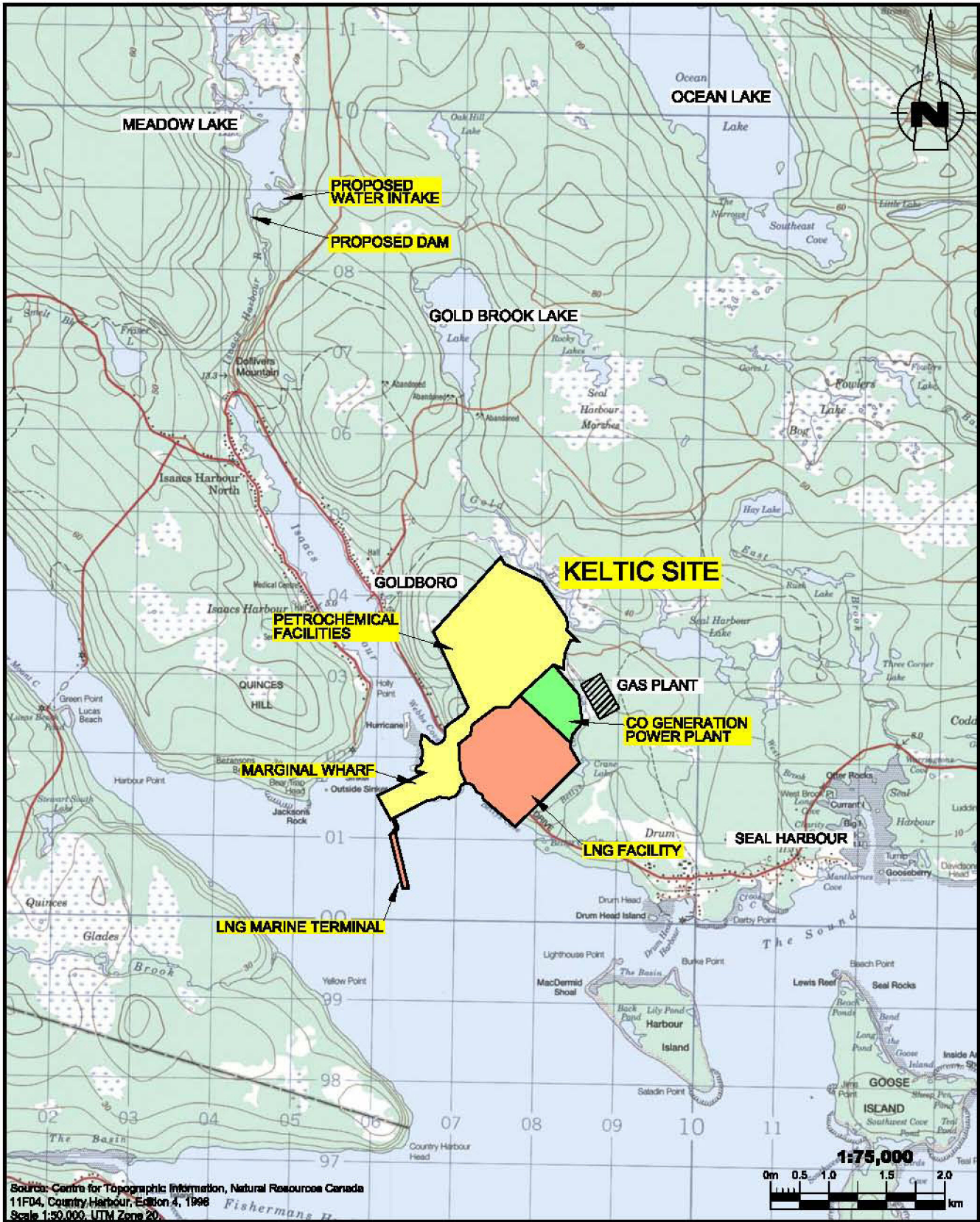
FIGURE No. 1.1-1B KELTIC PETROCHEMICALS INC. PROJECT LOCATION AND BASIC LAYOUT JULY 2006
