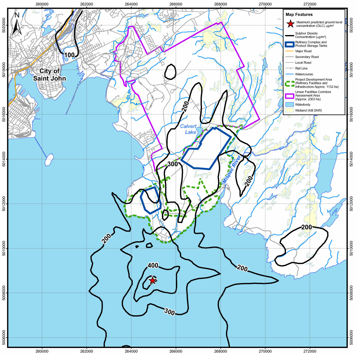
Figure 7.4 Maximum Predicted 1-Hour Sulphur Dioxide (SO 2 ) Concentrations Cumulative Environmental Effects Case
