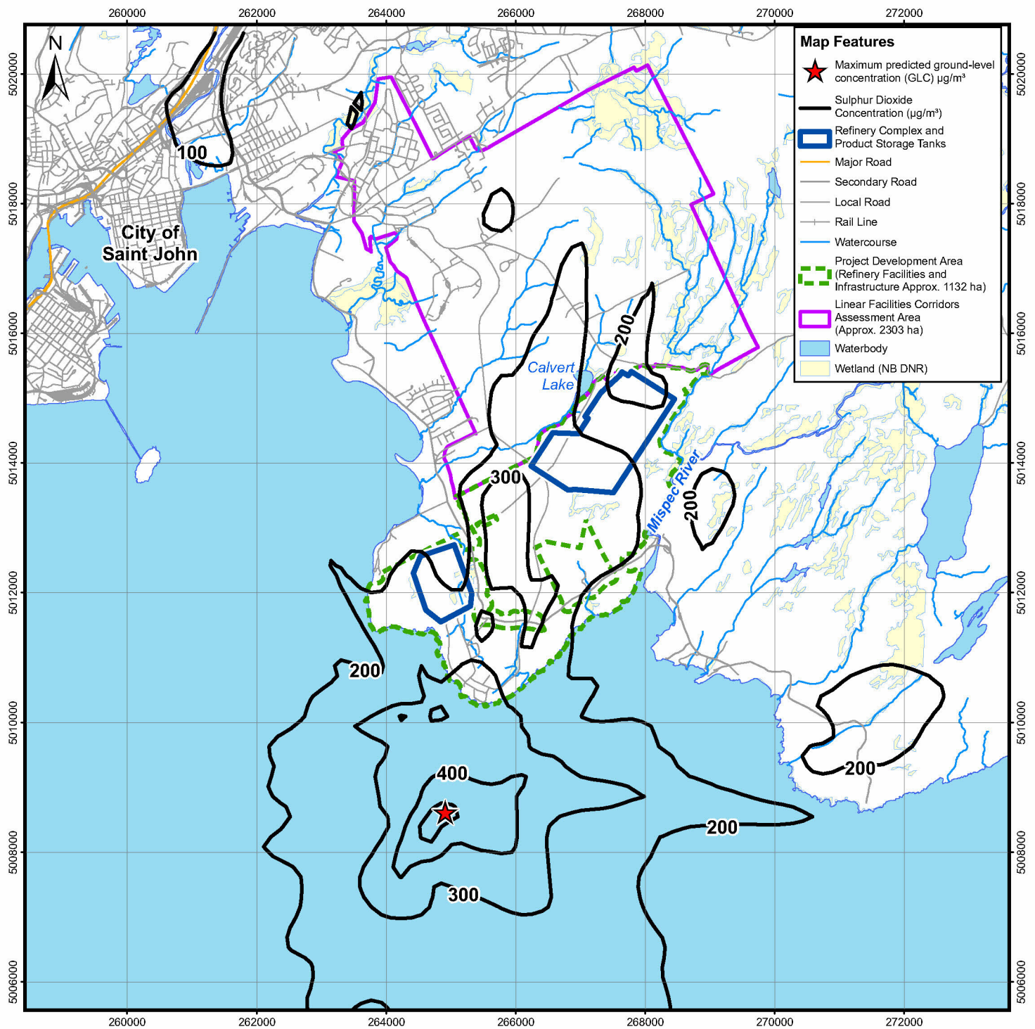
Figure 7.6 Maximum Predicted 1-Hour Sulphur Dioxide ( \text{SO}_2 ) Concentrations Marine Terminal and Other Marine-Based Infrastructure
