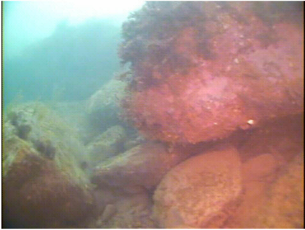
Figure 10.31 Substrate in Area A Boulder in upper right quadrant of figure is covered in pink encrusting coralline algae ( Lithothamnion sp.) and the red seaweed, sea oak ( Phycodrys rubens ). This figure is typical of this type of substrate found in all of the survey areas and at varying water depths.
