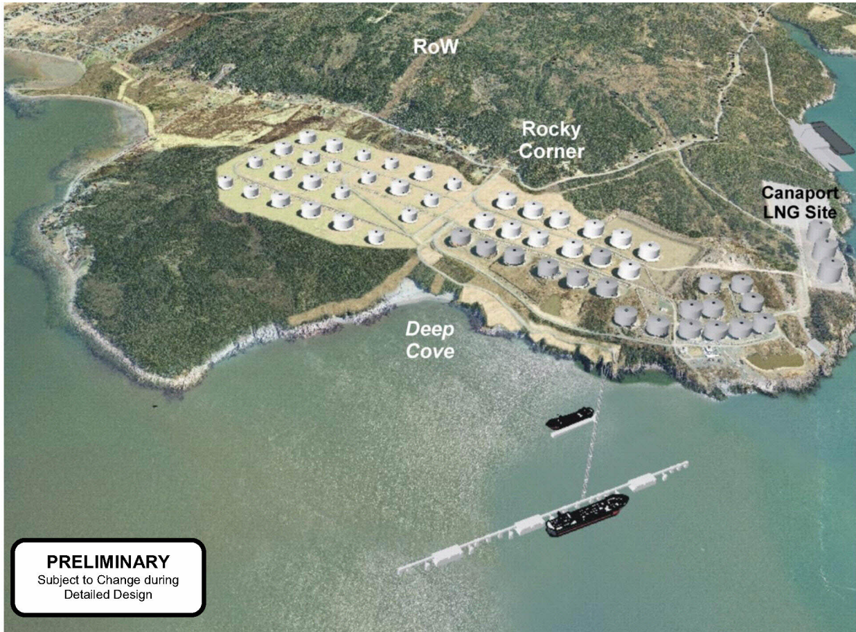
Figure 3.3 Conceptual Rendering of Marine Terminal (Jetty and Trestle Structure)
