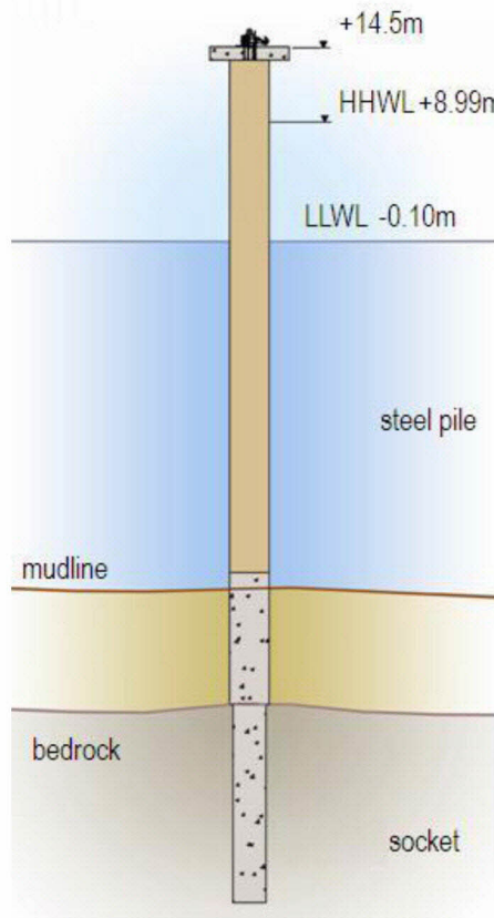
Figure 3.6 Schematic of Pile Construction
