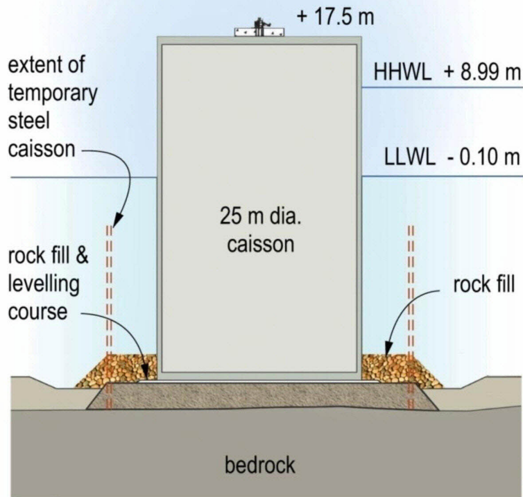
Figure 3.5 Schematic of Typical Caisson Construction (Temporary Steel Caisson Method)
