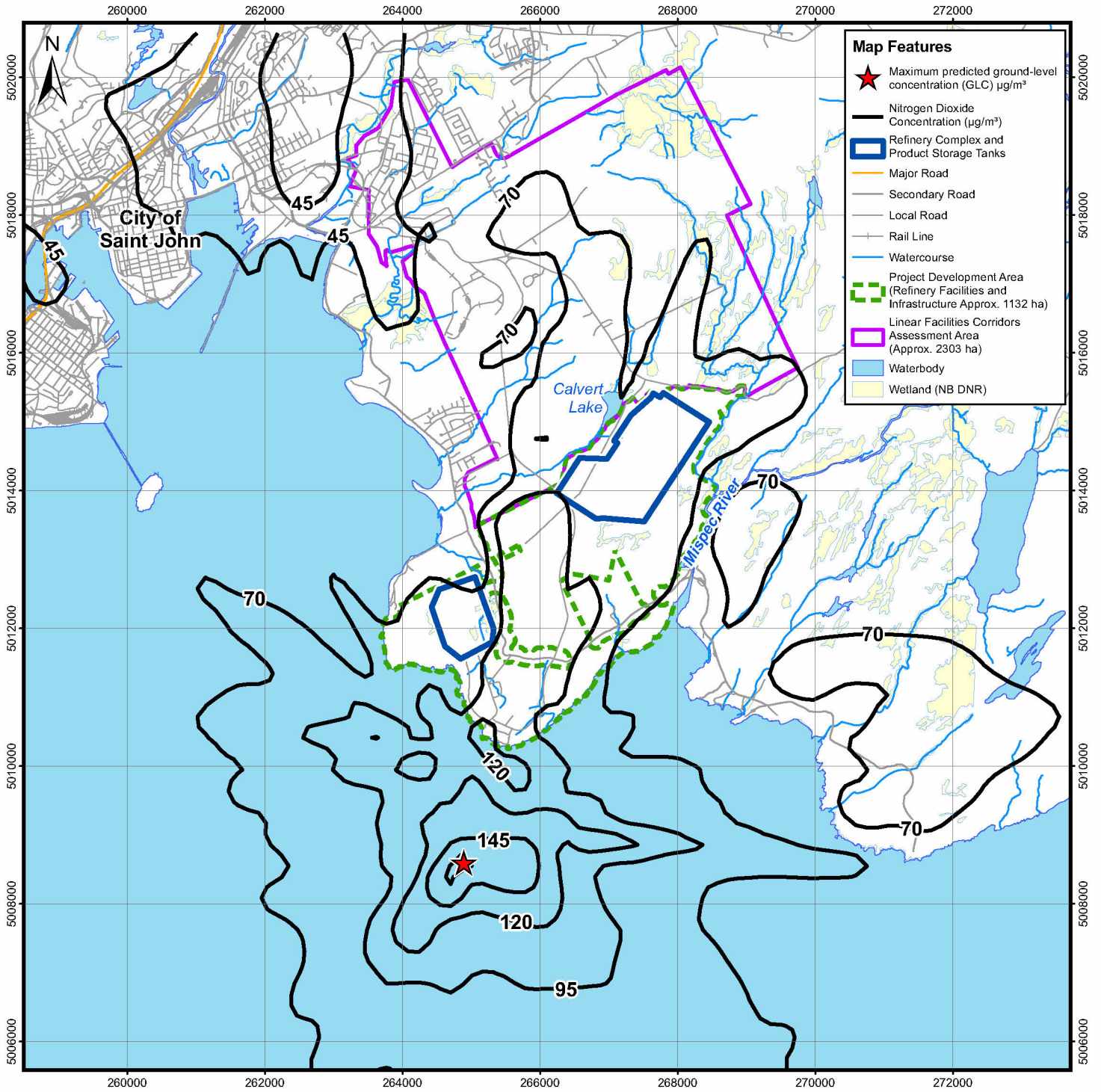
Figure 7.5 Maximum Predicted 1-Hour Nitrogen Dioxide ( \text{NO}_2 ) Concentrations Marine Terminal and Other Marine-Based Infrastructure
