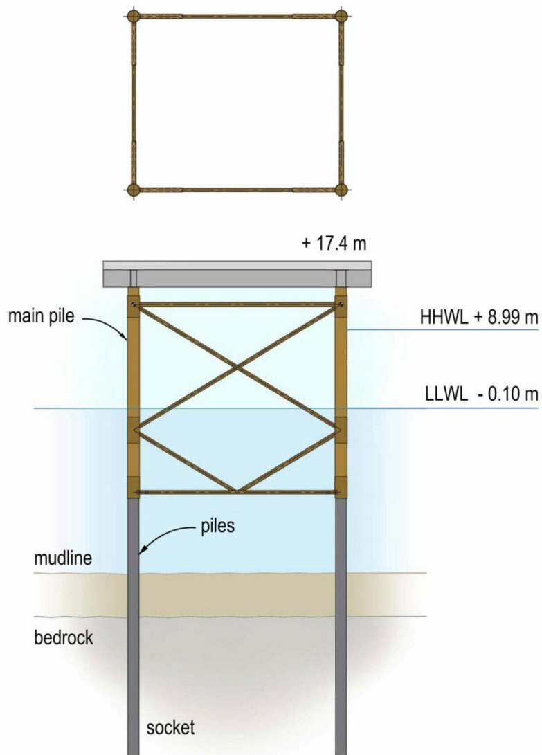
Figure 3.4 Schematic of Typical Jacket Structure
