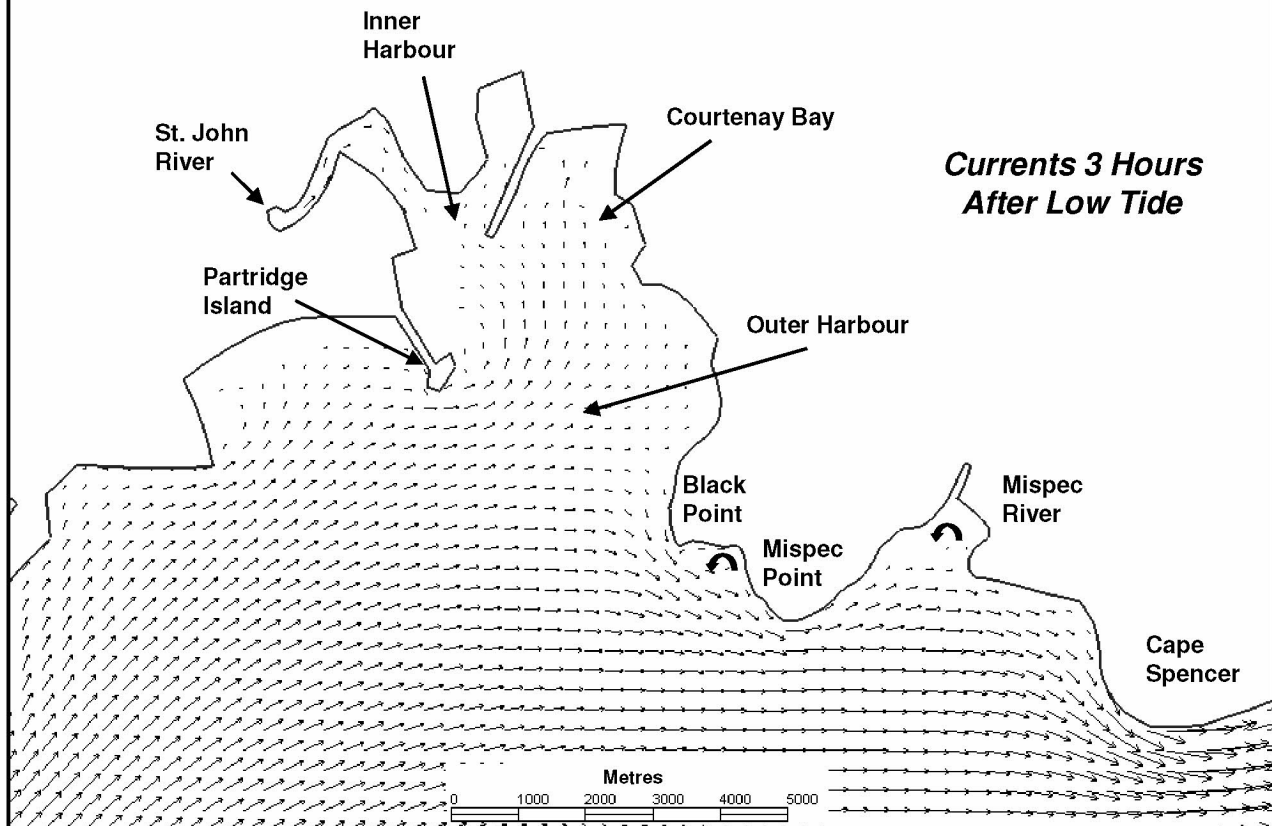
Figure 10.17 NATECH Model of Simulated Currents for the Saint John Harbour
