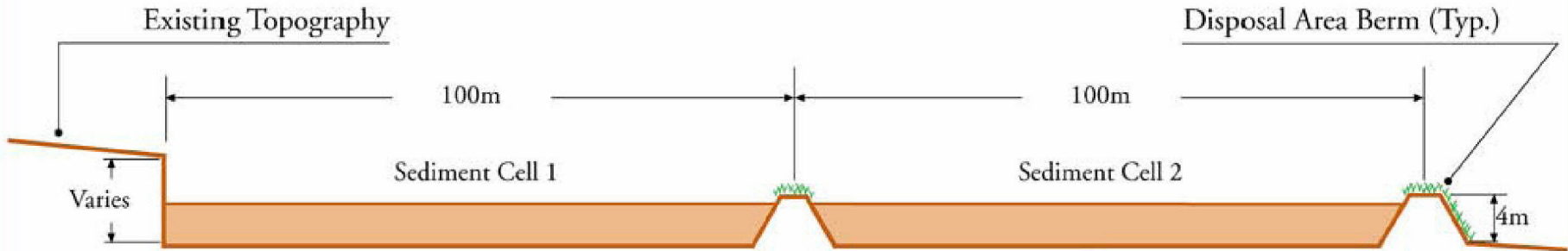
Section SD-1 - Sediment Disposal Area Years 1 - 20
