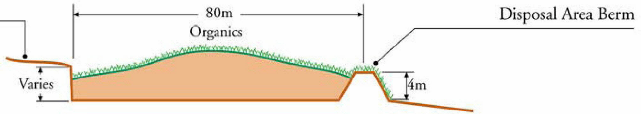
Section OD-1 - Organic Disposal Area Years 1 - 30
