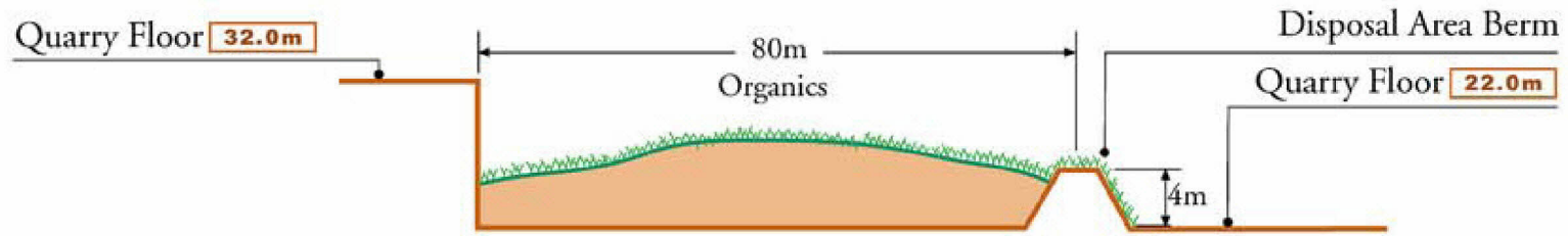
Section OD-2 - Organic Disposal Area Years 31 - 49
