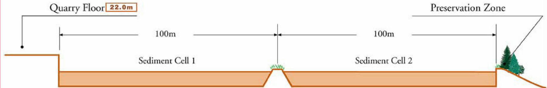
Section SD-2 - Sediment Disposal Area Years 21 - 49
