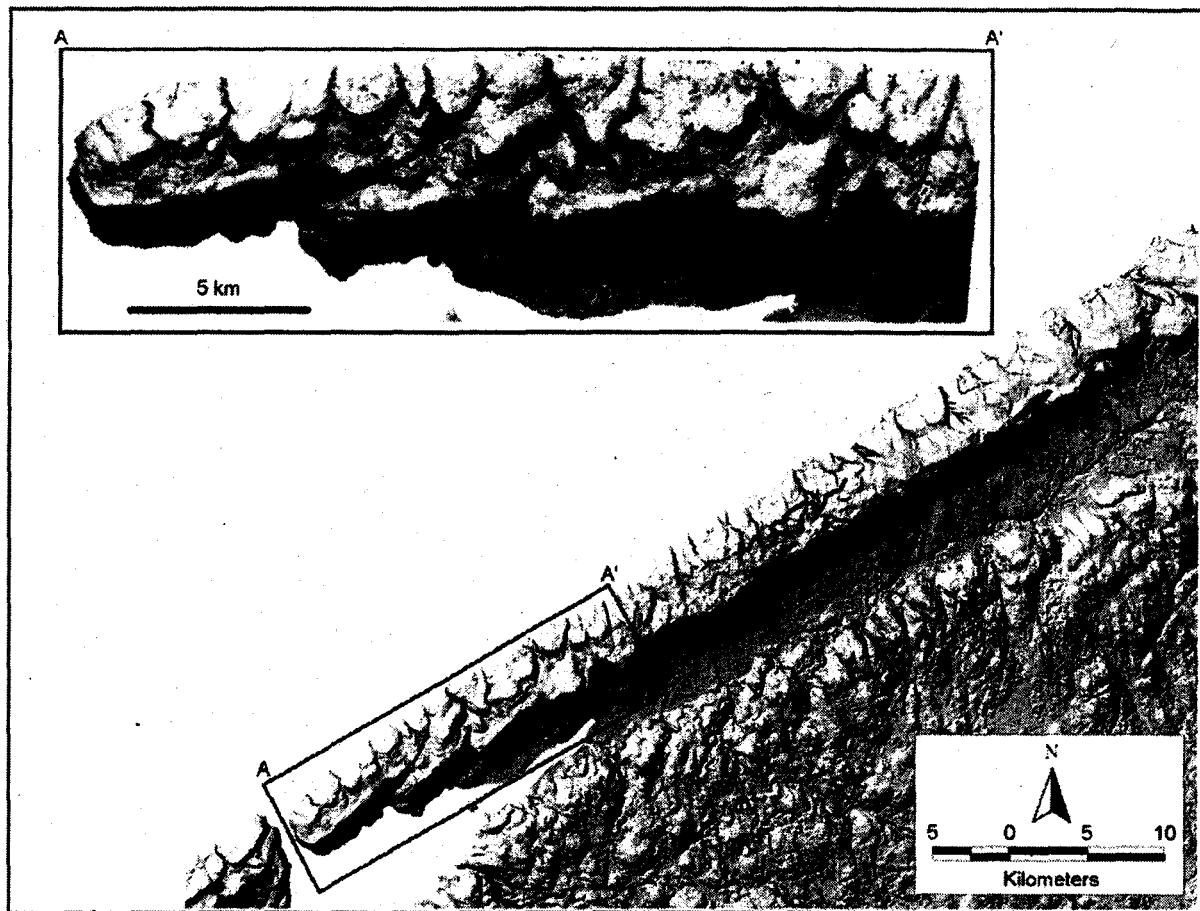
Figure 7. Digital elevation map with grey scale coloration of part of the Annapolis Valley region between Annapolis Royal and Digby. Note that the area northeast of Digby Gut has been enlarged to show detail. The North Mountain Basalt forms a prominent topographic feature that clearly indicates the extent of this unit. The enlarged area shows that the thick (i.e. ca. 150 m), lower flow unit is overlain by the middle flow unit and that multiple thin flows are recognizable and enhanced due to differential weathering of zeolitized flows.
