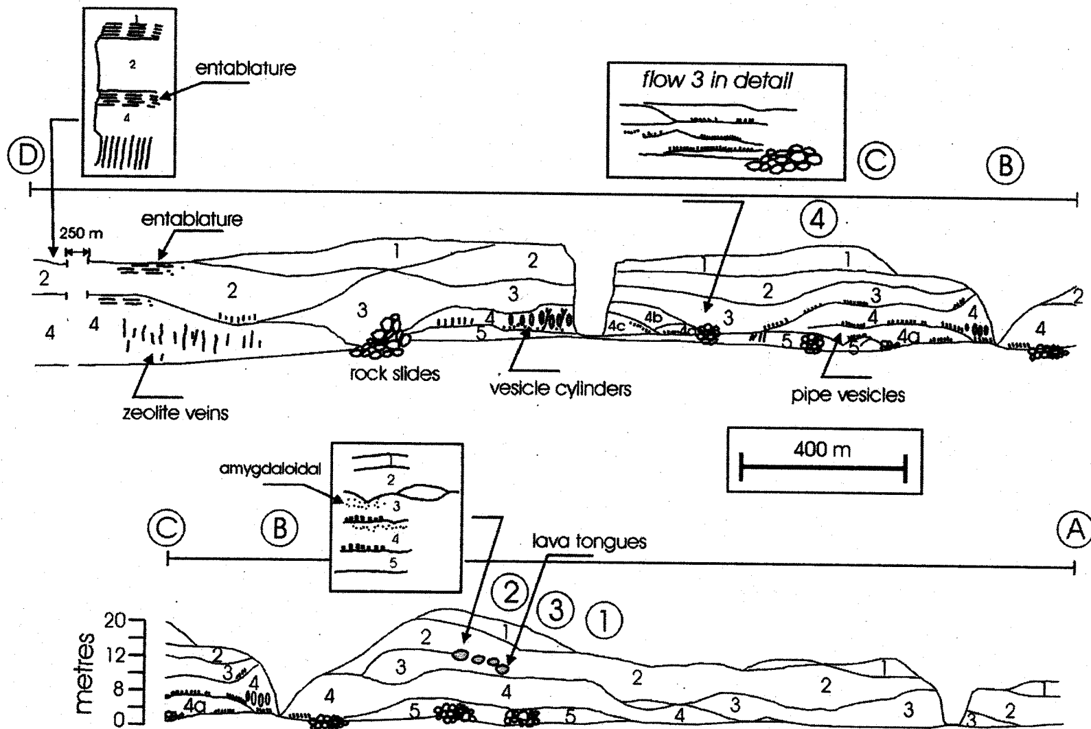
Figure 5. Long section parallel to the coastline from Margaretsville northeast towards Bishop Creek (between sections a and b in Figure 3) which shows flows of the middle flow unit of the North Mountain Basalt in the cliff section. Note that flow 5 outcrops extensively at low tide, but is not shown in the section. The section commenced northeast of Lighthouse Point past the wharf and a concrete retaining wall in front of a cottage. The section was generated by noting flow stratigraphy every 50-100 m along the traverse line parallel to the coastline. Note vertical exaggeration.
