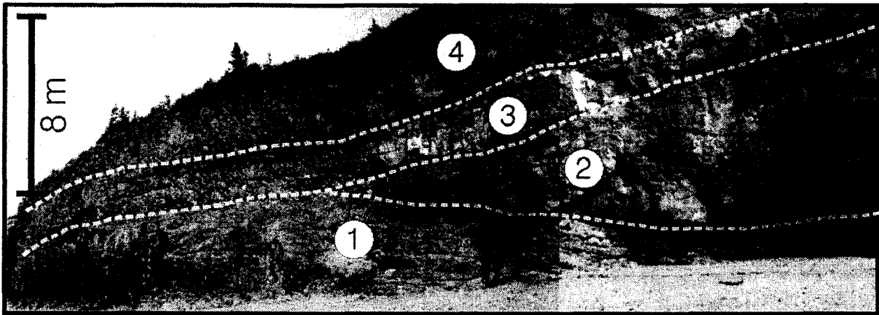
Figure 4. Photo mosaic of MFU flows at Victoria Harbour (facing southeast) showing occurrence of four basalt flows (numbered 1-4). Note that flow 2 pinches out to the northeast, but that it re-appears along the section.
