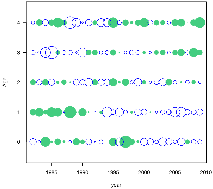
Figure 4: Normalized catch residuals ((\text{obs}-\text{pred})/\text{std}) from area 1. The area of the circle is proportional to the absolute value of the normalized residual, the empty circles correspond to positive residuals, and the shaded circles correspond to negative residuals.
