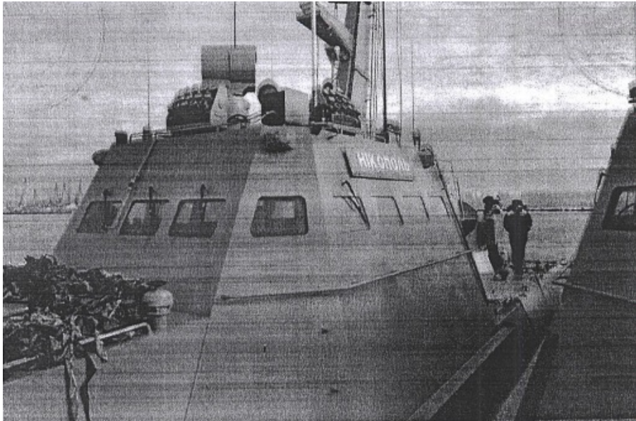
Picture 2: Left side view of the small armoured artillery boat “Nikopol”.
